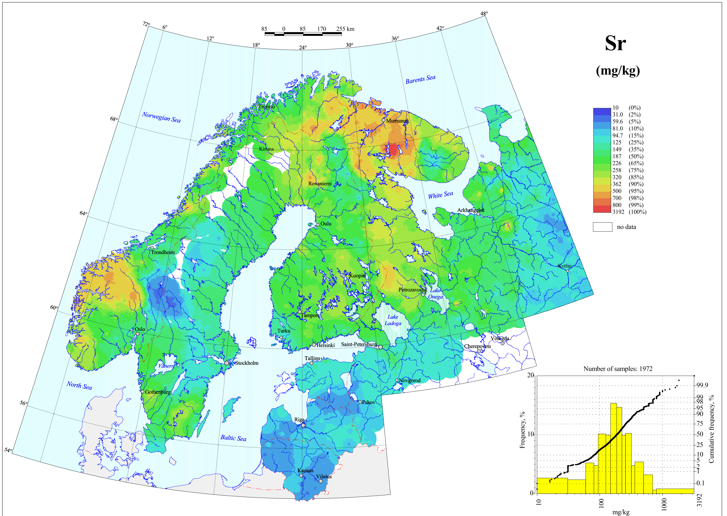
Strontium in C-horizon, Grain Size <2 mm, Total Content
